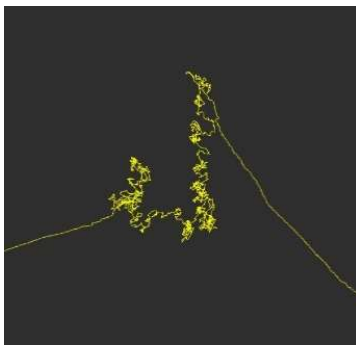
Fig. 12 Failure of LiDAR odometry in the middle of a grass field Source: author.
