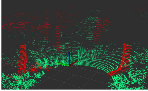
Fig. 8 Traversability estimation of a point-cloud using DeepLabv3 ResNet101/TraversabilityClouds Source: author.
