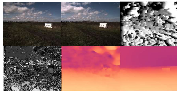
Fig. 11 Depth estimation from an uncalibrated stereo-pair of images. First row (left-to-right): left camera image, right camera image [2], depth estimated by ASW algorithm; Second row: SGM, ACVNet trained on KITTI [31, 32] dataset, HITNet trained on Middlebury dataset Source: [2] (input data), author (processing).
