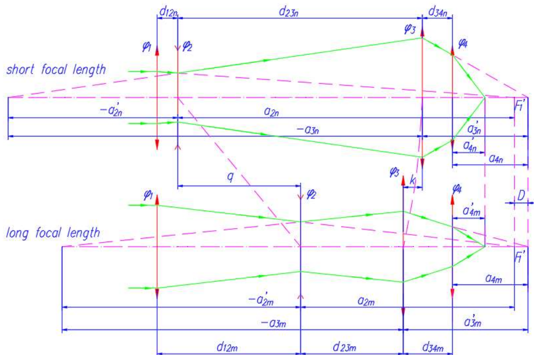
Fig. 1 Diagram of the principle of positive compensation in the IR zoom optical system
