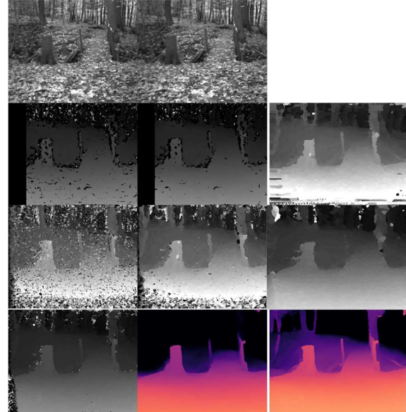
Fig. 10 Depth estimation. First row (left-to-right): left camera image, right camera image [15]; Second row: depth estimated by BM [16], SGBM [17], ASW [18] algorithms; Third row: AD-Census V1 [19], SAD [20], ZNCC [21]; Fourth row: SGM [22], ACVNet [23] trained on SceneFlow [24] dataset, HITNet [25] trained on Middlebury [26, 27, 28, 29, 30] dataset Source: [15] (input data), author (processing).
