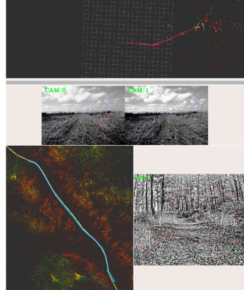
Fig. 14 Visual odometry using OpenVINS [35] - top: on Rellis-3D [2] dataset (red - ground-truth trajectory, purple - OpenVINS odometry); bottom: on our dataset (yellow - ground-truth trajectory, cyan - OpenVINS odometry) Source: author.
