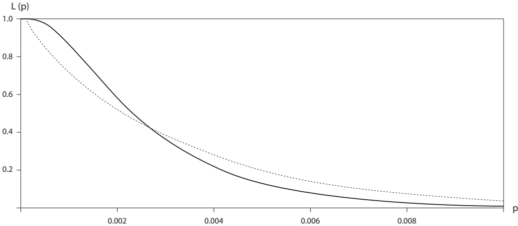
Figure 2 The OC of the AOQL plan for inspection by variables (98, 2.8715) and the OC of the AOQL plan for inspection by attributes (340, 0) – dotted
