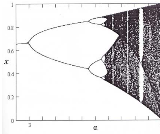
Figure 4. Bifurcation tree for a two-parameter model, \alpha = \beta
