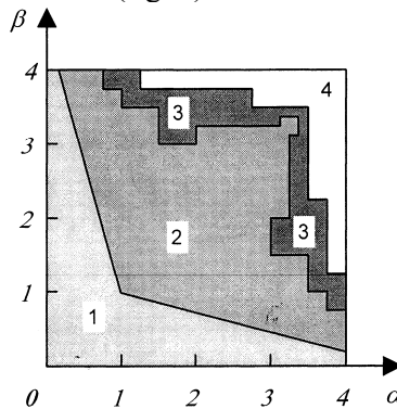
Figure 3. Results of numerical modeling of the system its parameters 0 \leq \alpha, \beta \leq 4 varied
