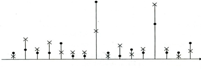
Figure 2. Distribution q of probabilities to select options of a complex system. (• is the distribution q^{k+\aleph} = \eta^1 ; × is the distribution q^{k+(\aleph-1)} = \eta^2 )
