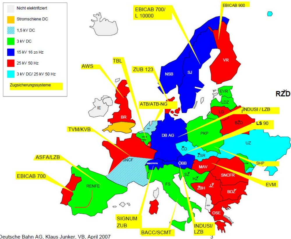
Figure 4: Current systems in Europe 39
