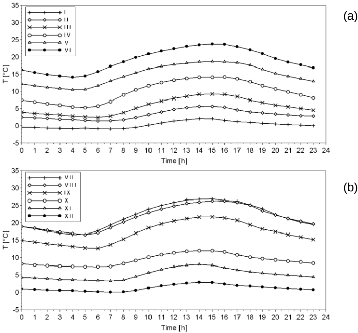
Figure 2: Daily air temperature at the station BTp in the months January–June (a) and July–December (b) in 2015–2016
