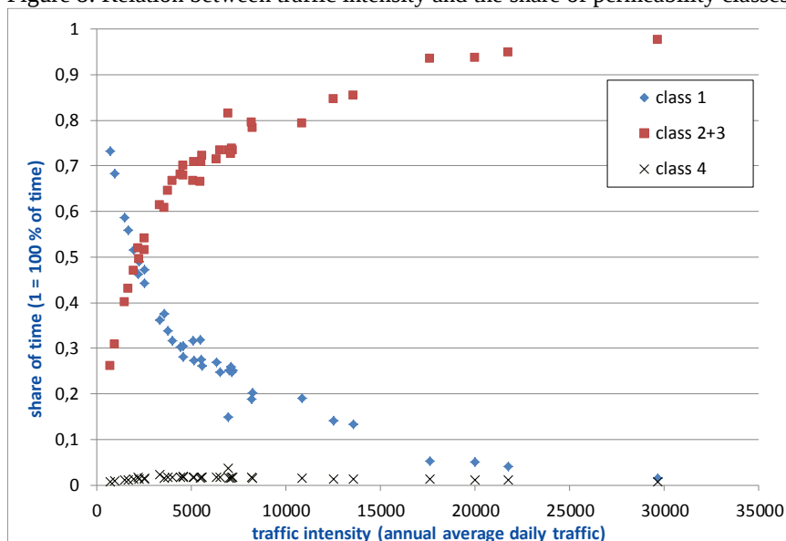
Figure 8: Relation between traffic intensity and the share of permeability classes
