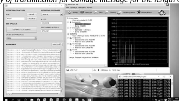
Figure 4: The test of delay of transmission for damage message for the length of datagram equal to 64bits
