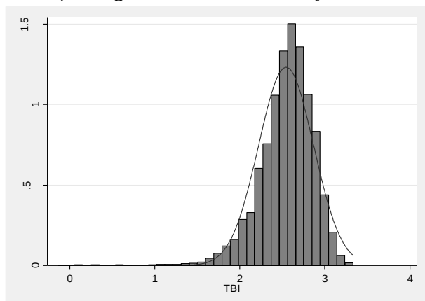
1) Histogram: Transformed Berry- Index
