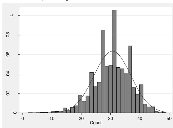
2) Histogram: Count Measure
