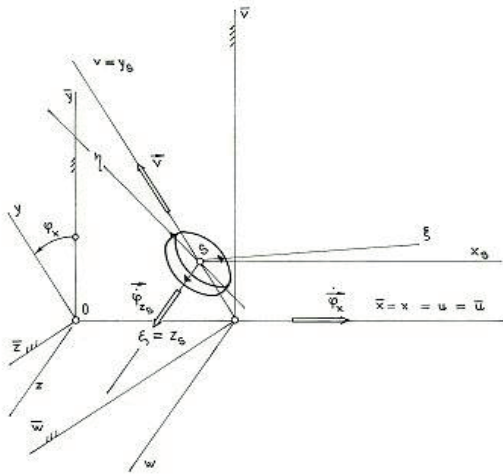
Figure 2 Coordinate system of the shaft
